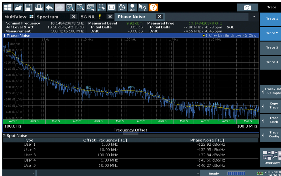
Phase noise at 10 kHz offset from a 10 GHz carrier: typ. -133 dBc (1 Hz)
